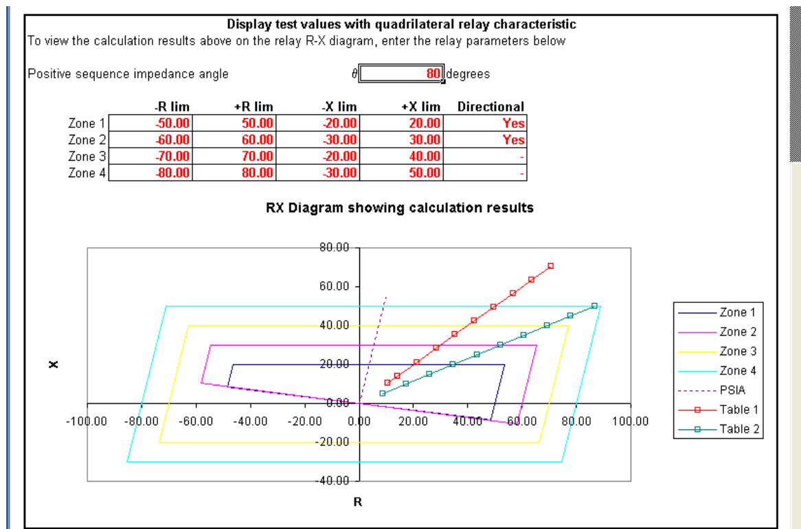
Figure 12. Results display on R-X diagram
