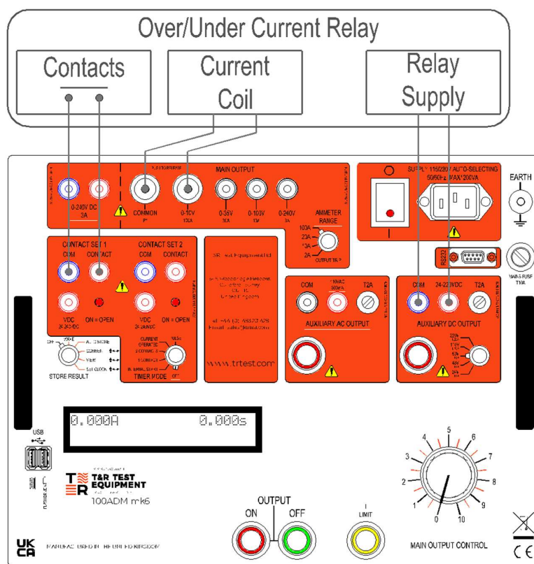
Figure 3.4 Connections for current pick-up/drop-off test
