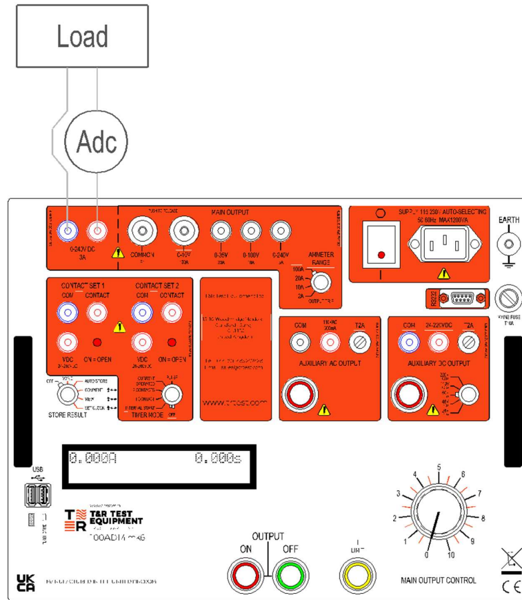
Figure 2.3 Main output dc current
