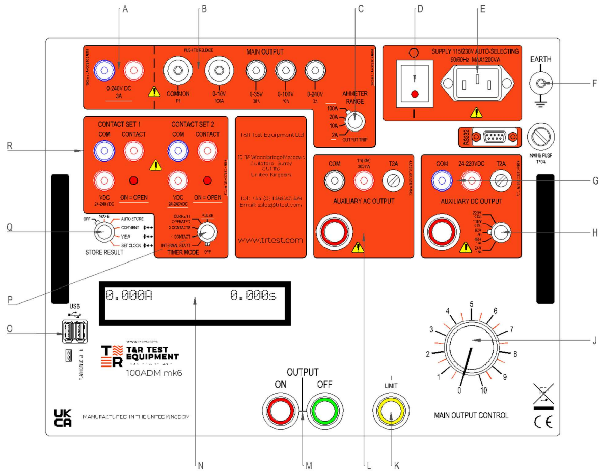
Figure 1.1 100ADM mk6 front panel
