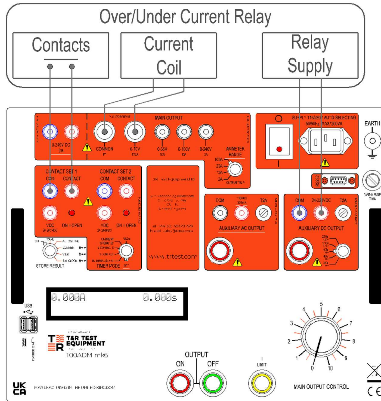
Figure 3.3 Connections for current drop-off test
