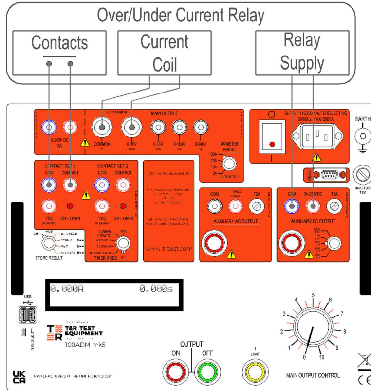
Figure 3.1 Connections for current pick-up/drop-off test
