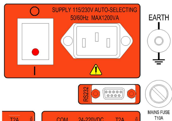
Figure 1.6 Mains input
