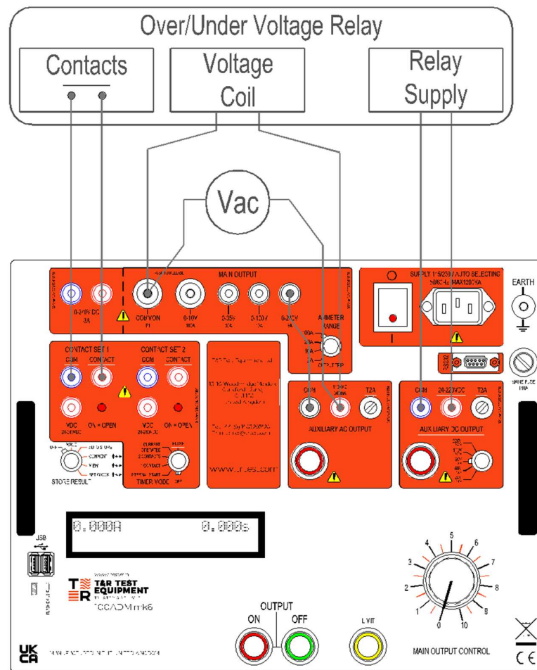
Figure 3.8 Over-voltage with timing
