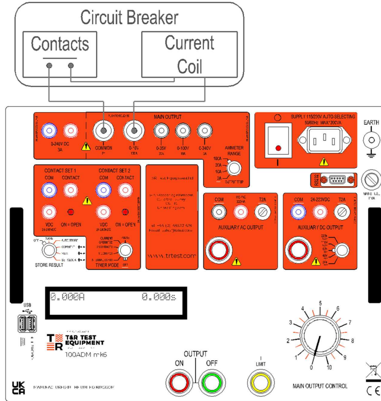
Figure 3.10 Connections for testing circuit breakers
