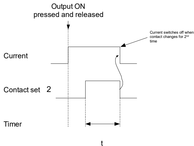
Figure 1.10 Single contact mode using contact set 2 (C2)
