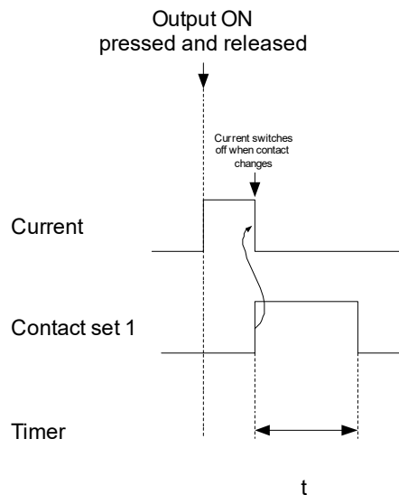
Figure 1.9 Single contact mode using contact set 1 (C1)
