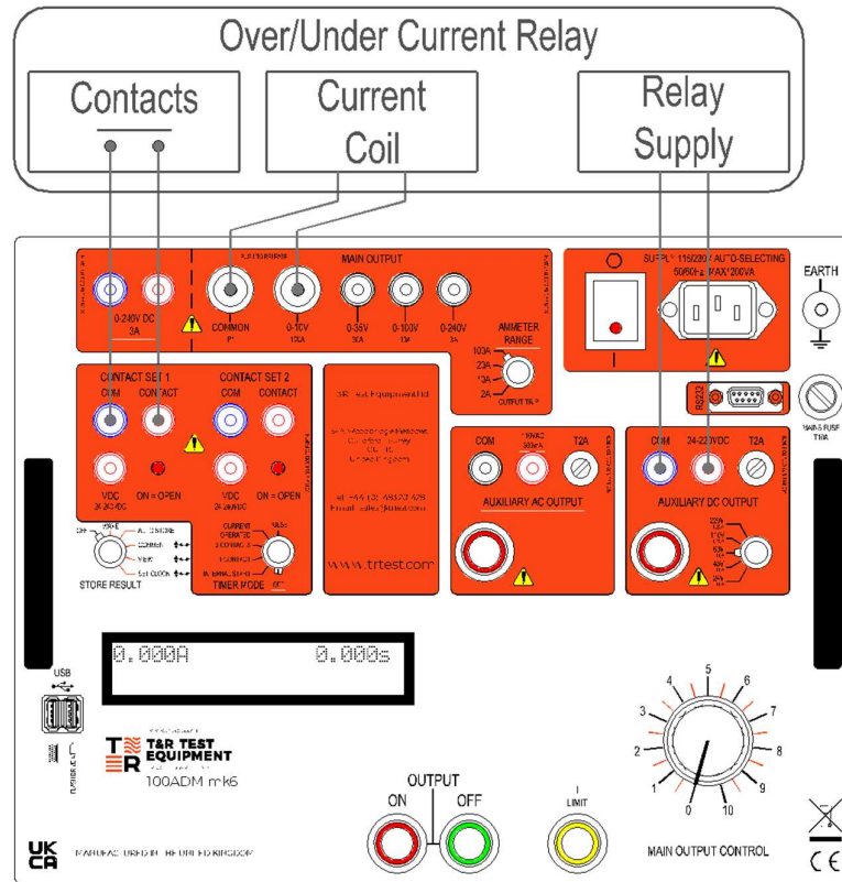
Figure 3.2 Connections for over-current timing
