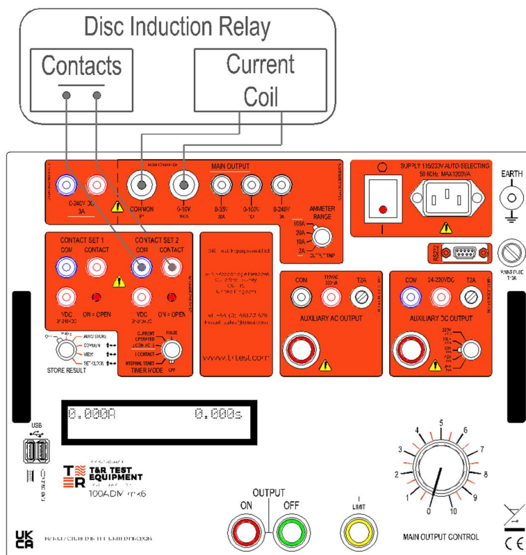
Figure 3.12 Connections for run-back timing
