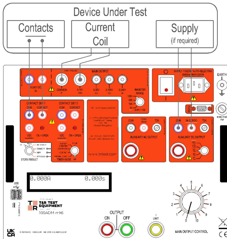
Figure 2.2 Main output ac current with timing
