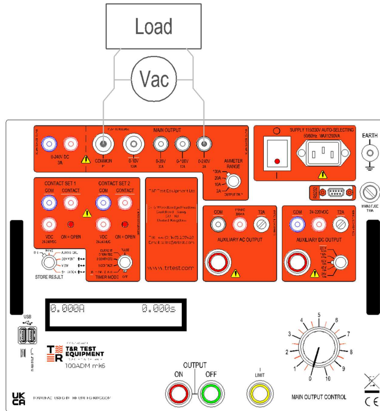
Figure 3.5 Connections for pick-up/drop-off test
