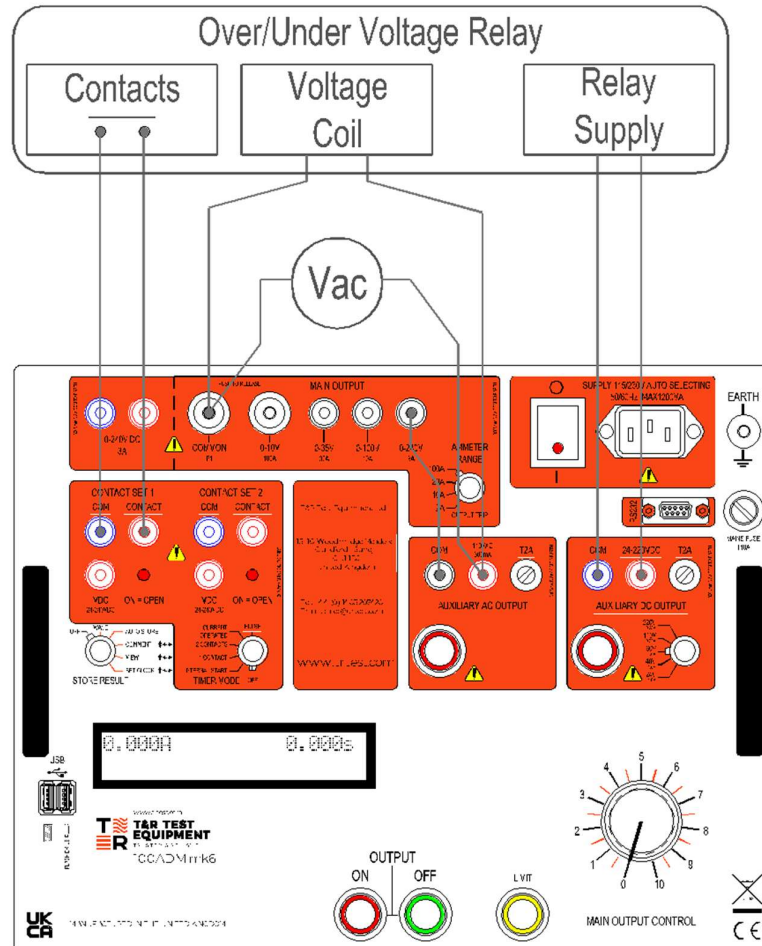
Figure 2.5 Voltage step
