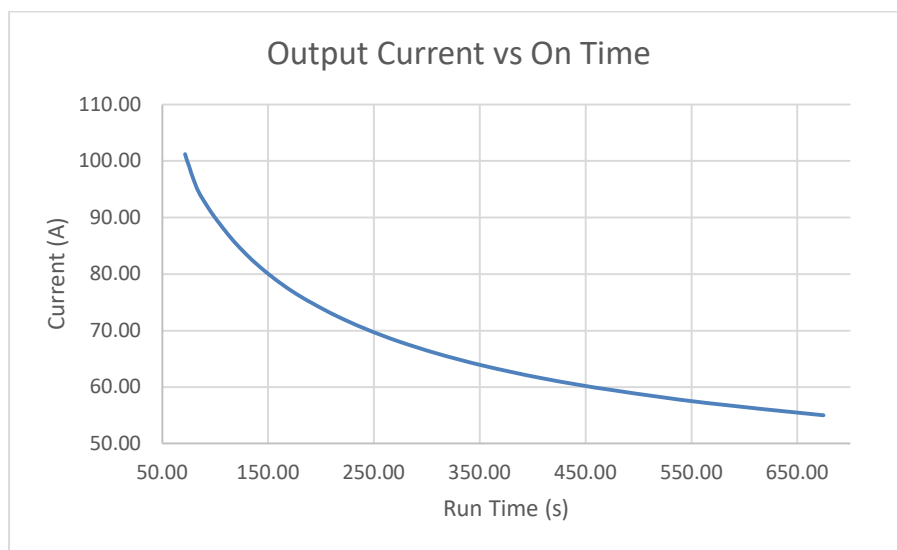
Figure 1.7 100ADM mk6 maximum 'on' times
