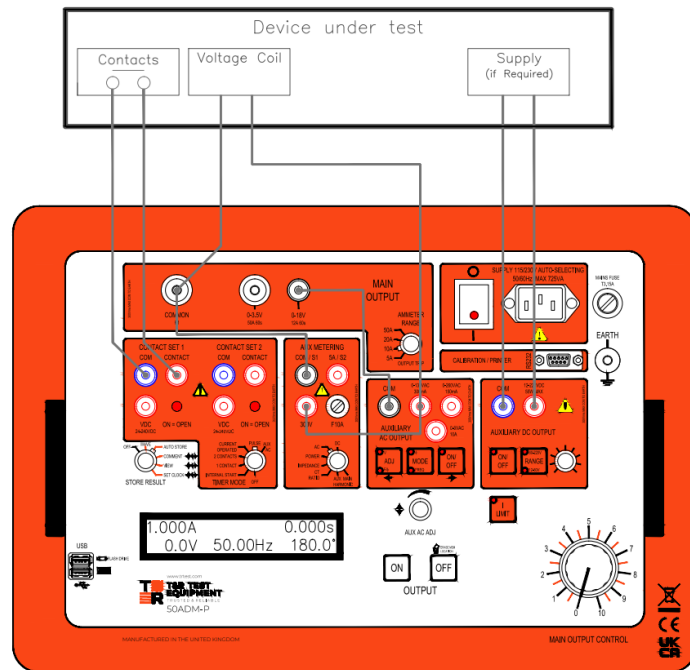
Figure 2.6 Voltage step
