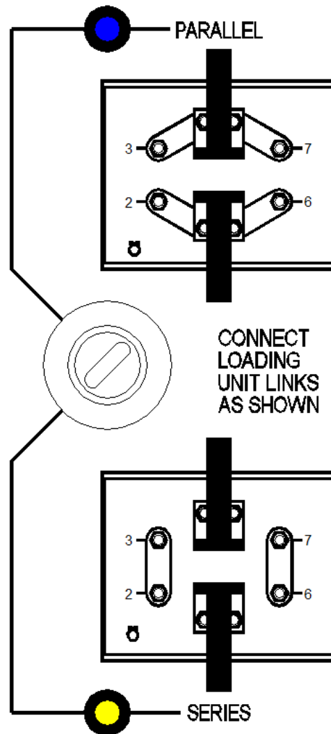
Figure 1.3.2 Loading unit series/parallel selection
