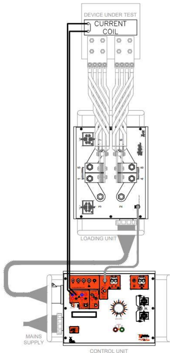
Figure 3.2 CU-Ps mk2 with over current device
