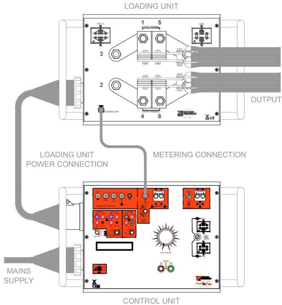
Figure 2.1 CU-Ps mk2 and loading unit connections
