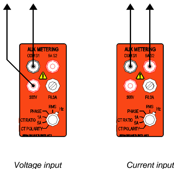
Figure 1.3.4 Auxiliary inputs
