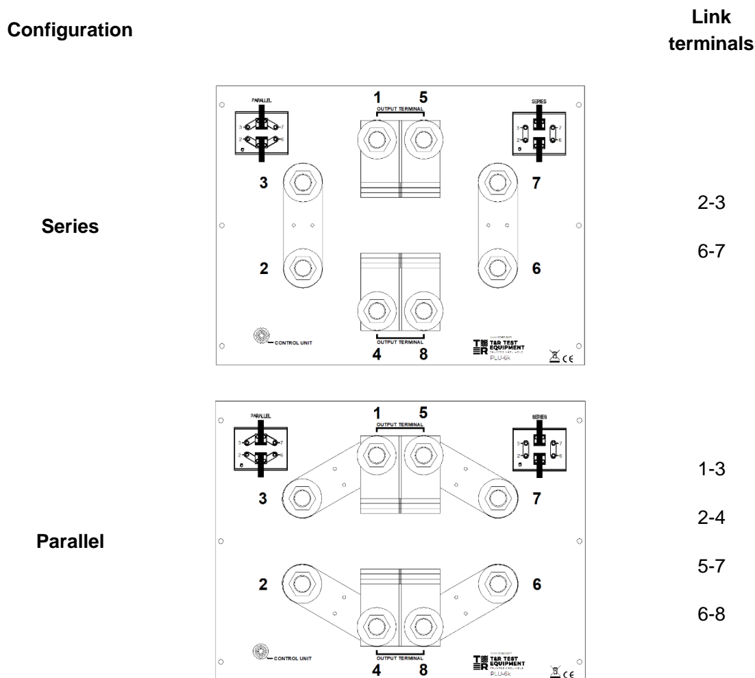
Figure 1.3.1 Loading unit series/parallel links arrangement
