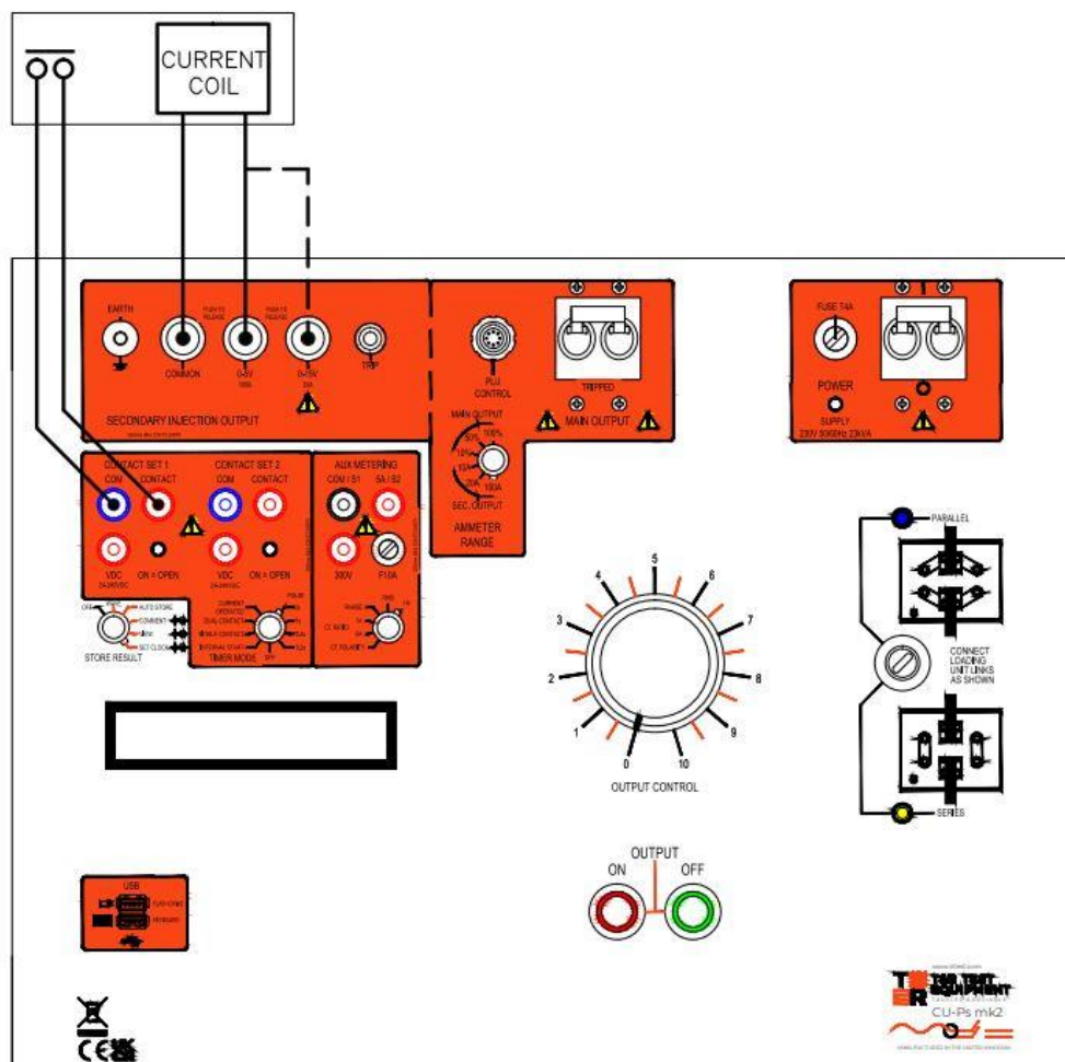
Figure 2.2 Secondary Injection Connections
