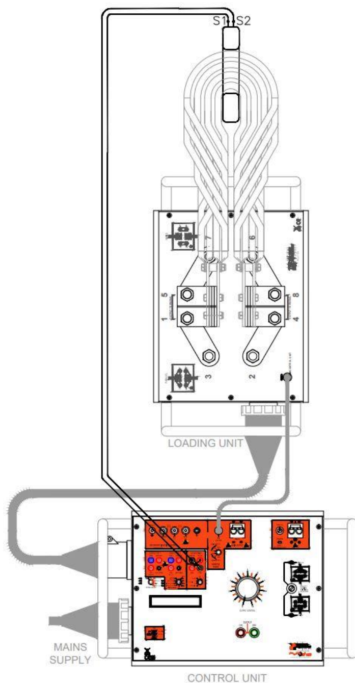
Figure 3.8 CU-Ps mk2 CT ratio/polarity
