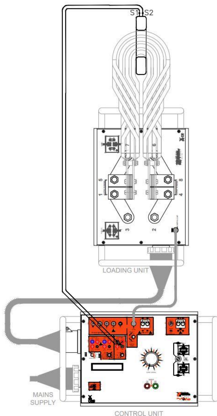
Figure 3.7 CU-Ps mk2 CT ratio/polarity
