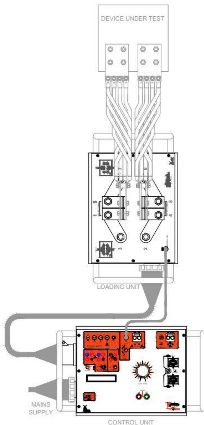
Figure 3.4 CU-Ps mk2 injecting into device with no auxiliary contacts
