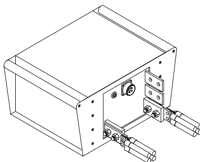
Figure 1.15 2000NAL connected to NLU
