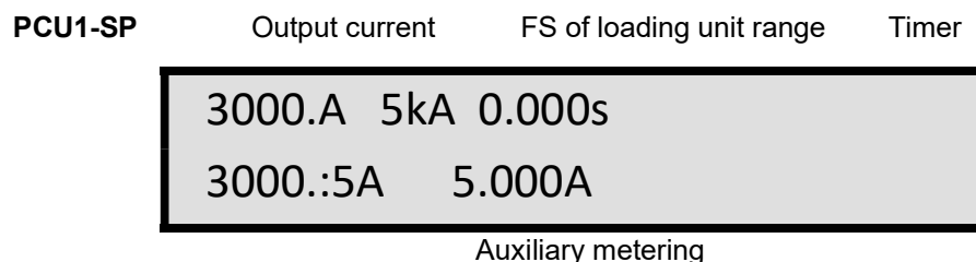
Figure 1.4 Normal values displayed on screen
