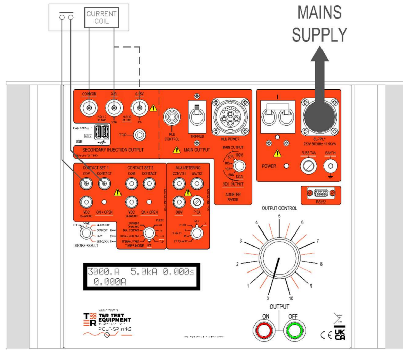
Figure 3.1 Secondary injection of over-current relay
