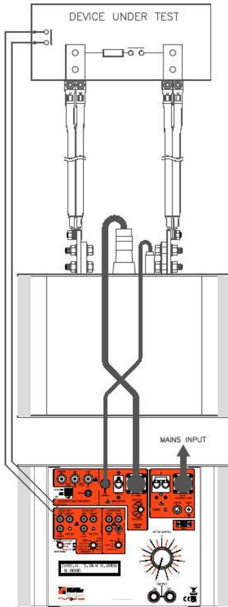
Figure 3.2 PCU1-SP with over current device
