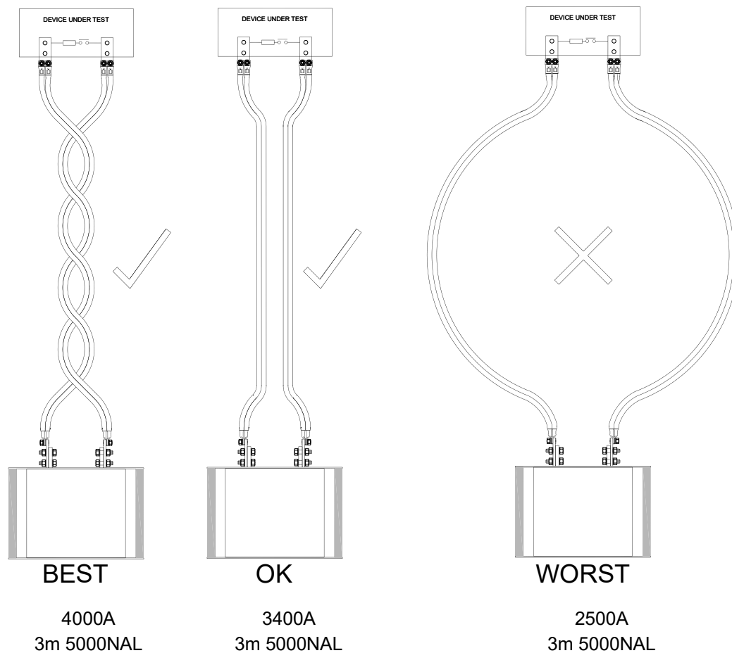
Figure 1.17 Effect of lead routing on maximum output current
