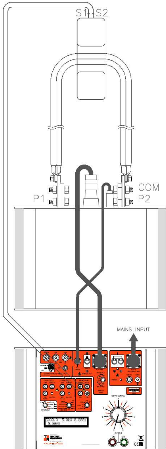
Figure 3.5 PCU1-SP CT ratio/polarity
