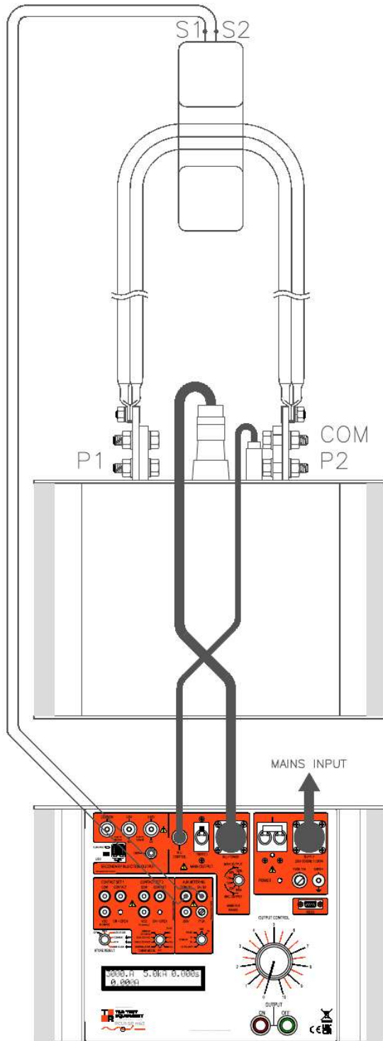
Figure 3.6 PCU1-SP CT ratio/polarity
